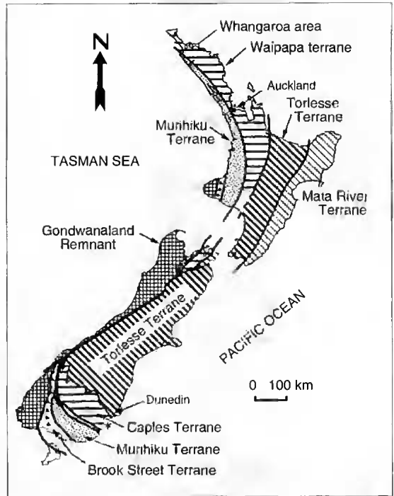
FIG. 2. — Map showing basement terranes of New Zealand and location of Whangaroa area (squared area) in the Waipapa Terrane, modified from Aita & Spörl (1992) and Roser et al. (1993). *, Bull Creek in the Caples Terrane.
